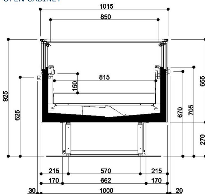
OPEN CABINET
