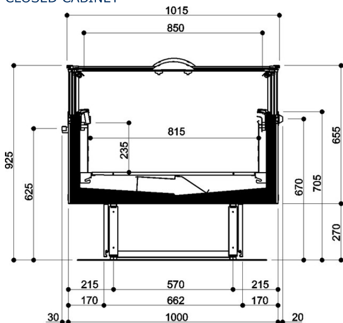
CLOSED CABINET
